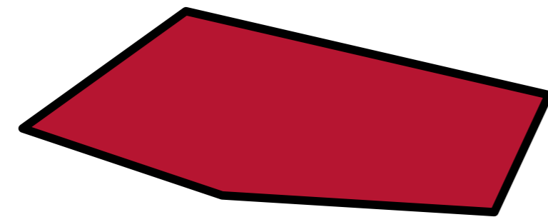
Polygone
