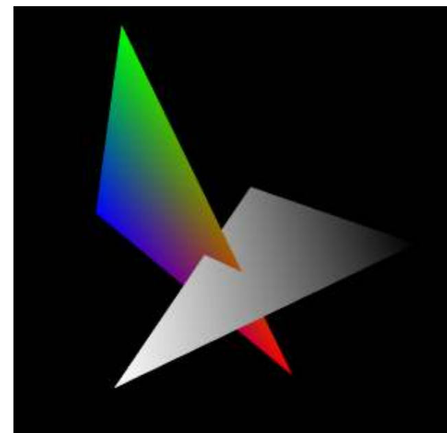
GL_TRIANGLES
