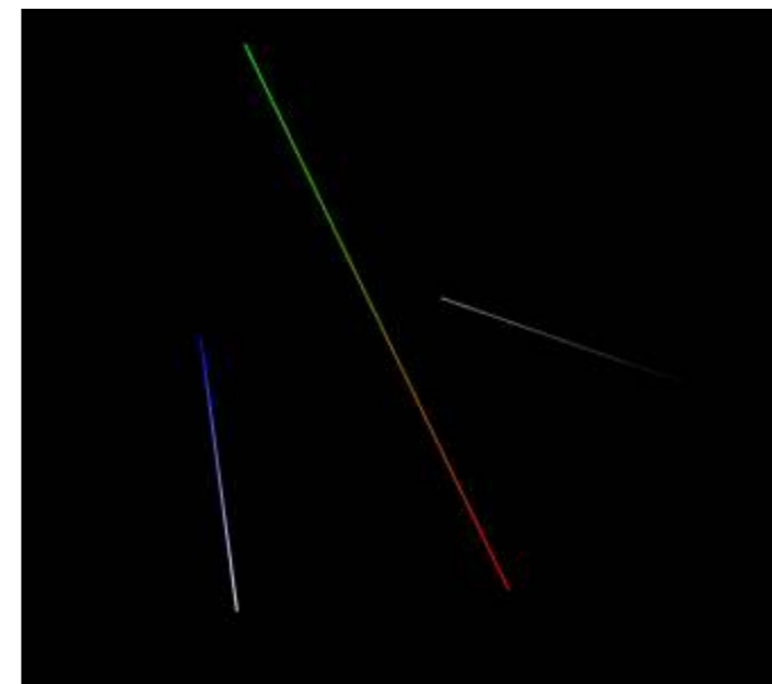
GL_LINES
